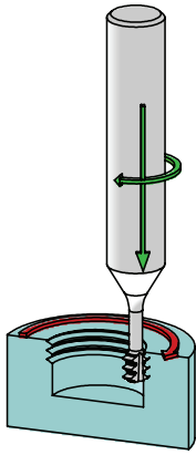
RIGHT HAND THREAD CONVENTIONAL MILLING
