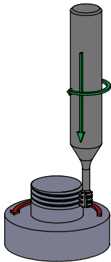
LEFT HAND THREAD CONVENTIONAL MILLING
