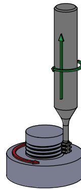
RIGHT HAND THREAD CONVENTIONAL MILLING
