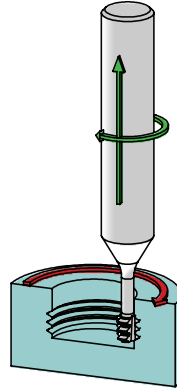
LEFT HAND THREAD CONVENTIONAL MILLING
