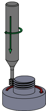
RIGHT HAND THREAD CLIMB MILLING
