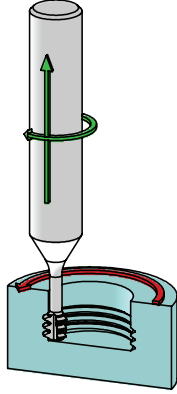
RIGHT HAND THREAD CLIMB MILLING
